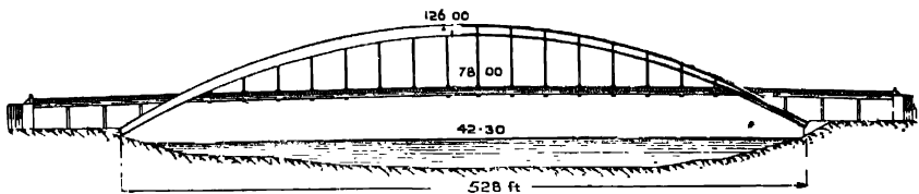
Fig. 371.—Dimensions: Bridge at Roche-Guyon over the River Seine, France.
